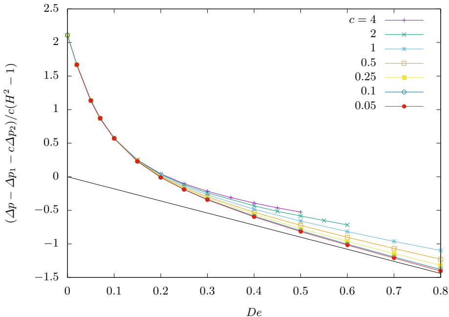
Figure 8: The effect of concentration. Plotted as a function of the Deborah number is (\Delta p - \Delta p_1 - c\Delta p_2)/(c(H^2 - 1)) , for c = 4, 2, 1, 0.5, 0.25, 0.05 , and for H = 2 . The solid black line is -\frac{9}{5}De .
