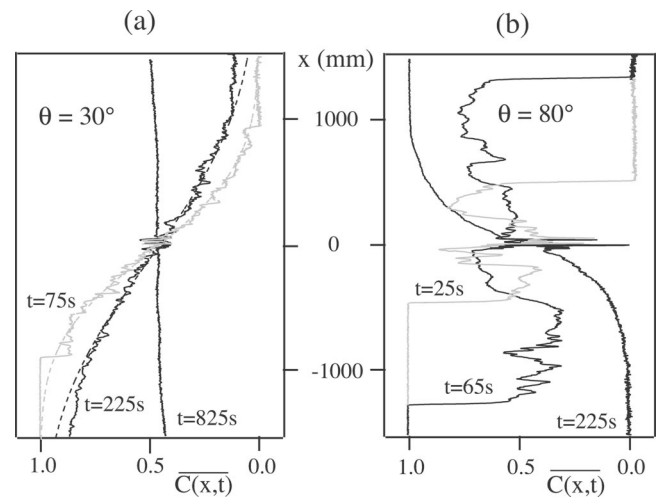
FIG. 3. Variations of \overline{C(x,t)} with distance from gate for At=4 \times 10^{-3} . (a) At times t=75 s (gray curve), 225 s, and 825 s for \theta=30^\circ (dashed lines are fits of the corresponding profile with an error function); (b) at t=25 s (gray curve), 65 s, and 225 s for \theta=80^\circ .
