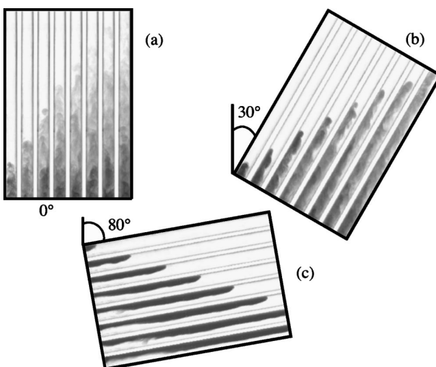
FIG. 2. Snapshots of video images obtained for At=4 \times 10^{-3} . (a) \theta=0^\circ , time interval between images \Delta t=7 s. (b) \theta=30^\circ , \Delta t=3 s. (c) \theta=80^\circ , \Delta t=3 s.
