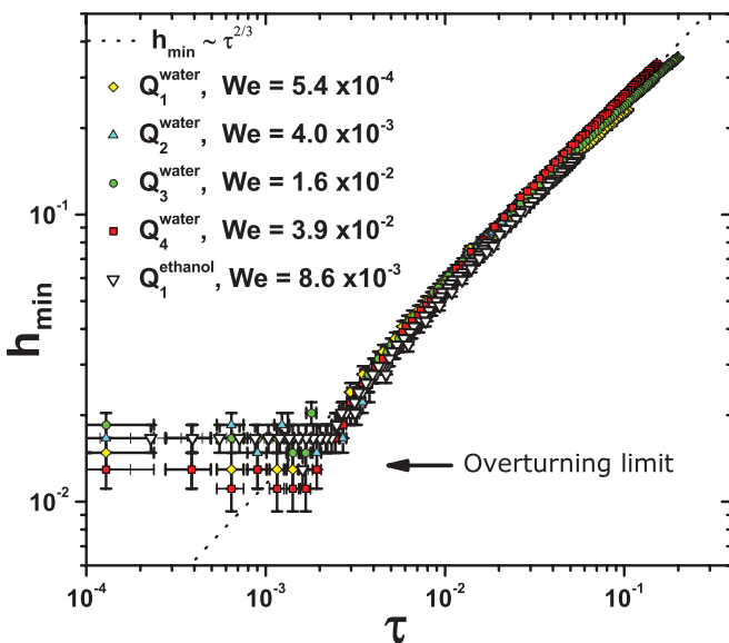
FIG. 4. (Color online) Experimental measurements of the minimum neck diameter h_{\min} in terms of the dimensionless time \tau to breakup for different fluids and different flows. Regardless of the condition of flow, within simple dripping the thinning follows a self-similar behavior. The dotted line represents the potential flow scaling law. The measurement of h_{\min} is limited by the overturning of the droplet surface.
