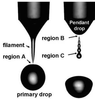
FIG. 1. Breakup regions found in dripping. The breakup at region A forms the primary drop, the breakup in region B detaches the filament from the pendant drop, and region C is found at one or several points of breakup within the filament.
