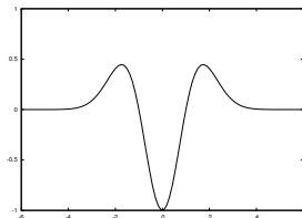
Figure: (a) Morlet wavelet with k = 6 . (b) Marr Mexican hat wavelet.
