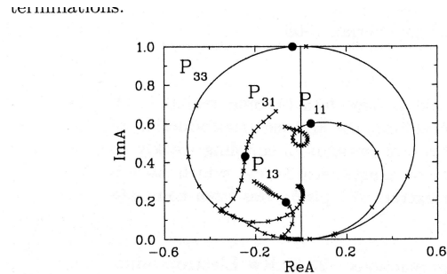
Fig. 2. Argand plots for P -partial-wave amplitudes from threshold (1080 MeV) to W = 2.5 GeV.
